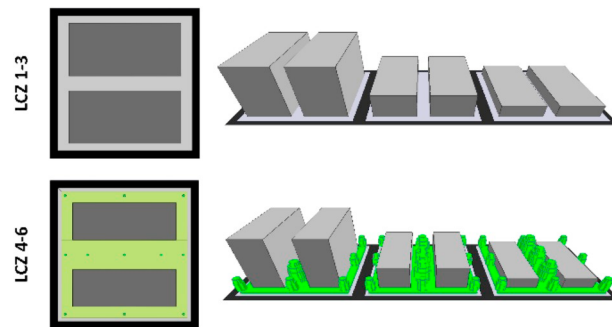
Fig. 18. Representation of the Standard LCZ tiles 1–3 and 4–6 gridded in 1 m resolution (they differ in building height only).
