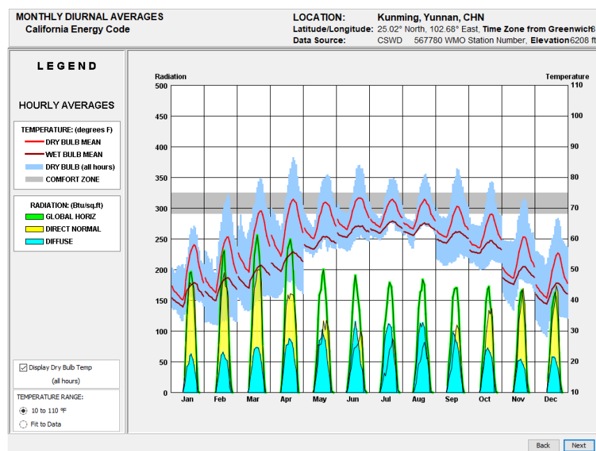
Figure 3. Climate data of Kunming (data source: EnergyPlus).
