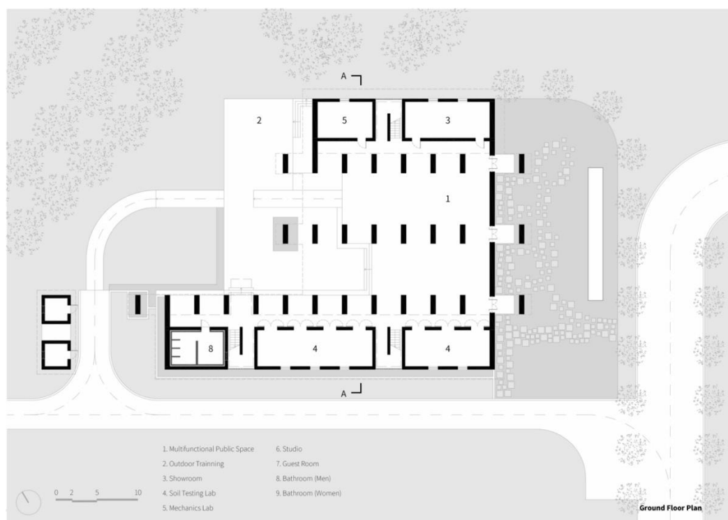
Figure 4. Ground floor plan of Terra Centre.
