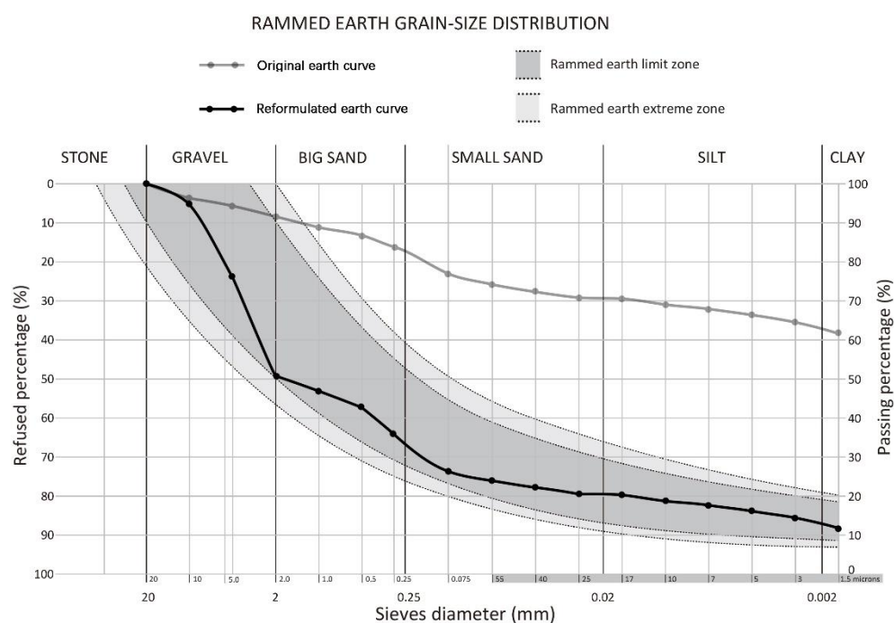
Figure 10. Soil sample analysis and optimization chart of the Terra Centre.
