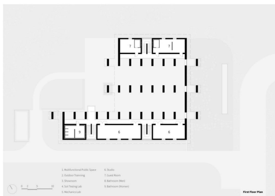
Figure 5. First floor plan of the Terra Centre.
