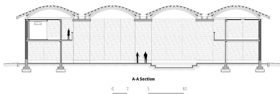
Figure 6. A-A section of the Terra Centre.
