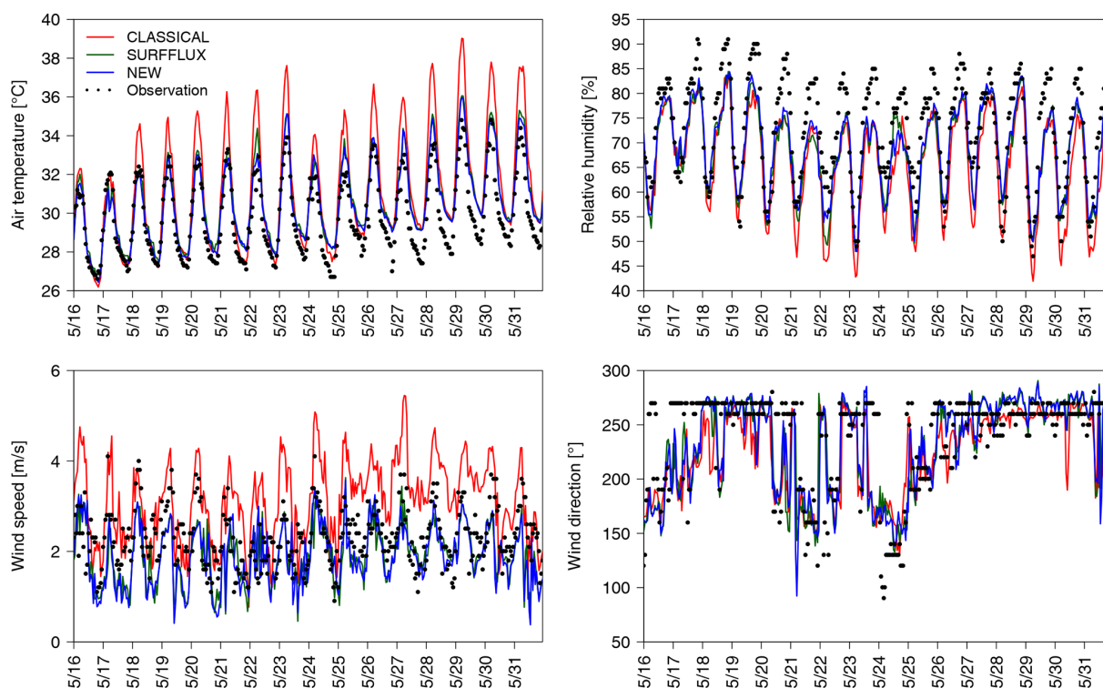
Figure 5. Time series (UTC) of simulated (D4) and observed meteorological variables at the KP station during HW2018.
