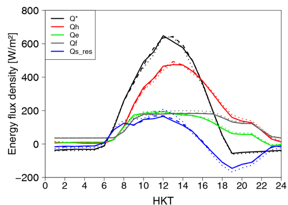
Figure 15. Daily cycle of the surface energy balance averaged for the entire duration of the heat waves and 1 \text{ km} \times 1 \text{ km} boxes centred on the King's Park and Hong Kong Park stations. Q_* is the net radiation, Q_h and Q_e are the upwelling turbulent sensible and latent heat fluxes, respectively, Q_f is the anthropogenic heat flux, and Q_s is the storage heat flux, which is diagnosed as the residual of the other fluxes. The continuous, dashed, and dotted lines correspond to the NEW, SURFEX, and CLASSICAL coupling approaches, respectively. HKT denotes Hong Kong Time.
