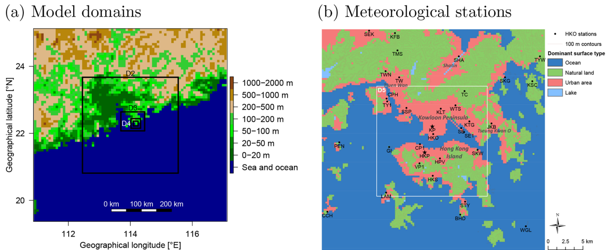
Figure 2. (a) The five nested Meso-NH model domains employed for the high-resolution simulation of the urban climate of Hong Kong. (b) Meteorological stations operated by the Hong Kong Observatory that are located within model domains D4 and D5. Model results will be presented in more detail at the starred stations (KP and HKP).
