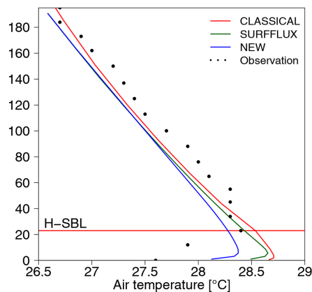
Figure 11. Vertical profiles of air temperature and wind speed at the KP station. H-SBL indicates the height below which for CLASSICAL the meteorological variables are taken from the SBL scheme.
